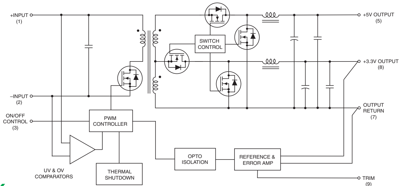
Figure 1. Simplified Schematic
